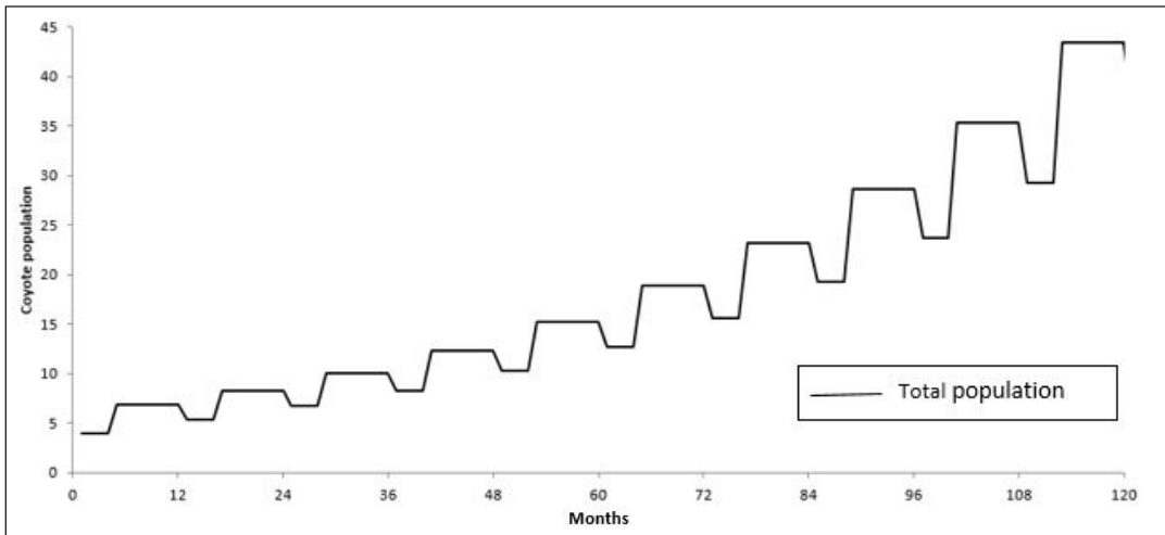
Figure 2. Initial evaluation of model output from the theoretical coyote ( Canis latrans ) population model in Texas, USA with no coyote mortality during a nondescript 10-year period. Simulations were conducted during 2016–2018.
